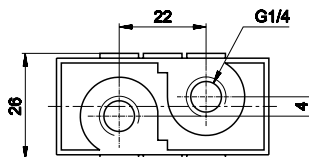
1 3/2 NC-NO
