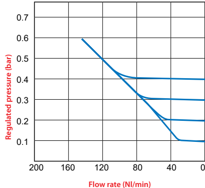
Relief characteristics
