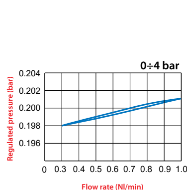
Pressure characteristics
