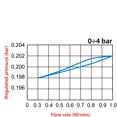
Pressure characteristics
