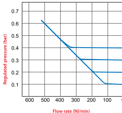
Relief characteristics
