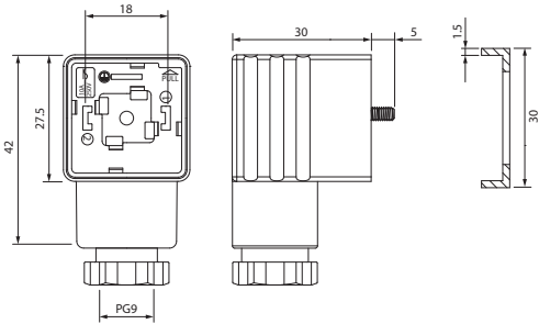
The dimensions are in millimeters (mm)
