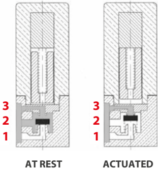
NORMALLY OPEN (NO) 3/2
