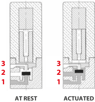
NORMALLY CLOSED (NC) 3/2
